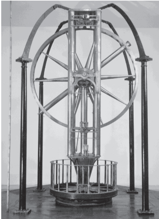
Fig. 2. The Palermo Circle by Jesse Ramsden (1730–1800), the greatest of the eighteenth-century instrument makers. With this instrument, Piazzi discovered Ceres in 1801. It was completed in 1789 after almost two years of intense work. The telescope has a 7.5-cm objective lens; the altitude scale (5 feet in diameter) was read with the aid of two diametrically opposed micrometer microscopes while the azimuth scale (3 feet in diameter) was read by means of a micrometer microscope. Recently refurbished (Brenni et al. , 2001; Chinnici et al. , 2001), all the parts of the telescope are original to the time of Ceres’ discovery, except for the eyepiece, which was replaced in 1855. Reproduced by permission of the Palermo Astronomical Observatory.
